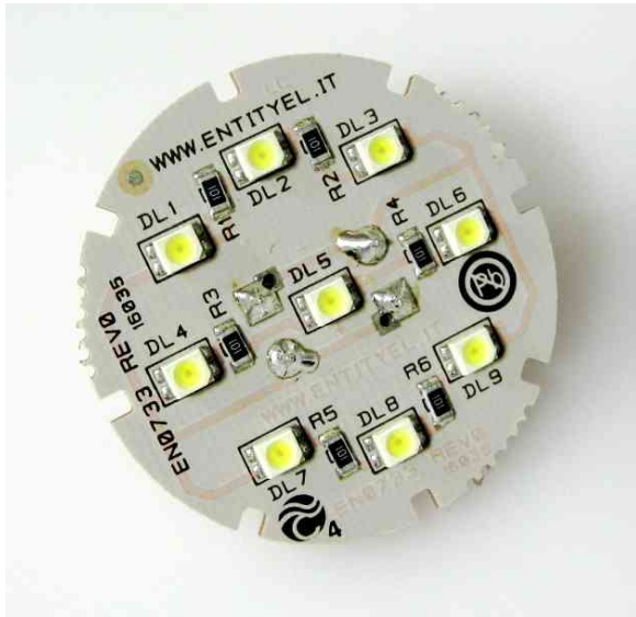
Modulo con 9 LED PLCC2, diametro 38 mm 9LED PLCC2 module, 38 mm diameter
